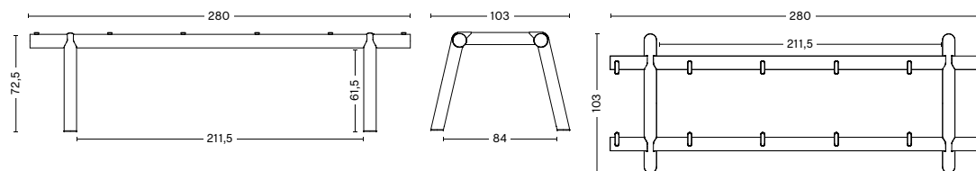
BOA TABLE FRAME Width 280 cm Depth 103 cm Height 72,5 cm
